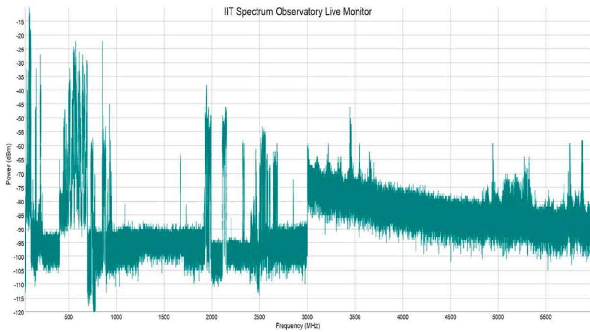
Figure 1 – Spectrum Usage in the City of Chicago – 5 October, 11:45 PM
